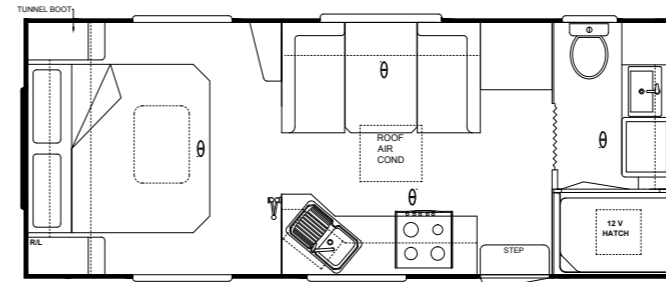
19'6" x 7'8" RD CARAVAN SHOWER
