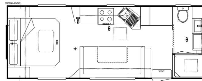
21' x 7'8" RD CLUB LOUNGE SHOWER
