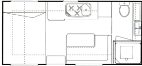
15'6" x 7' FD SHOWER
