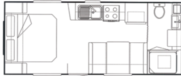
18'6" x 7'8" C/D SHOWER
