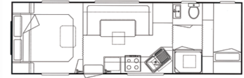
24'6" x 7'8" FD CLUB LOUNGE SHOWER BUNKS
